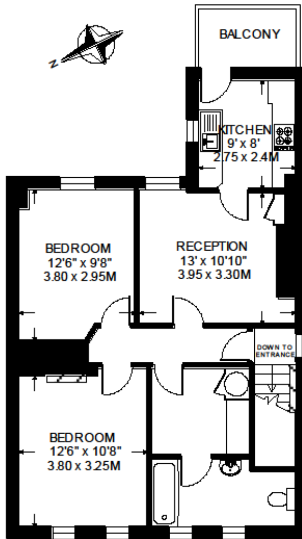
SECOND FLOOR
